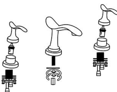
Two-Handle Widespread Faucet Installation
