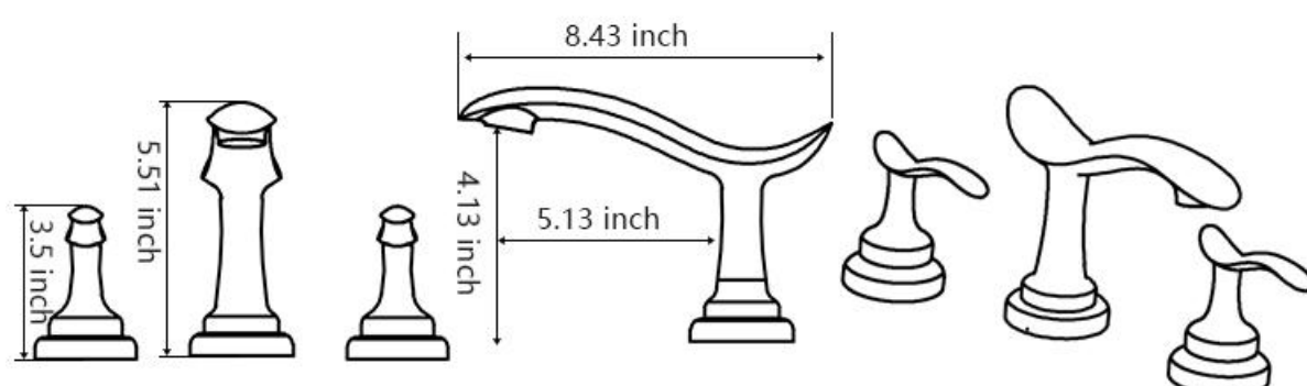
Two-Handle Widespread Faucet Installation
