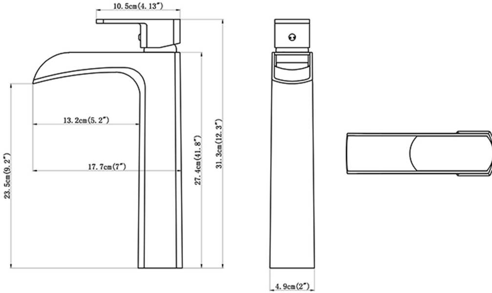
CRITICAL DIMENSIONS
