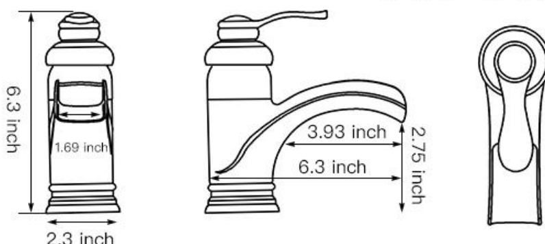
CRITICAL DIMENSIONS
