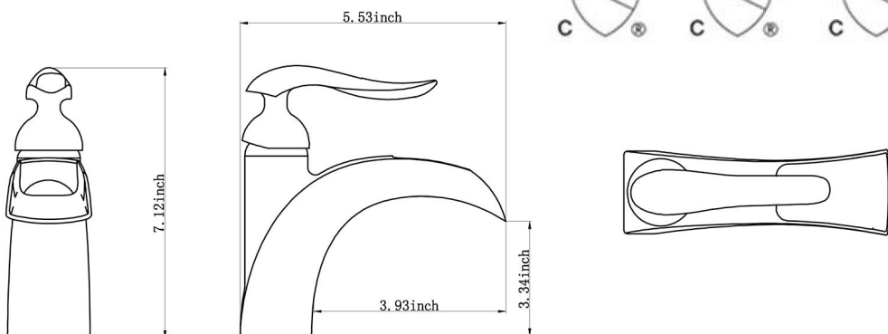
CRITICAL DIMENSIONS
