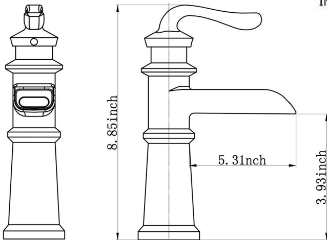
CRITICAL DIMENSIONS
