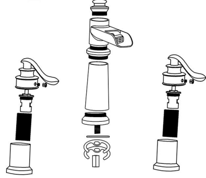
Two-Handle Widespread Faucet Installation
