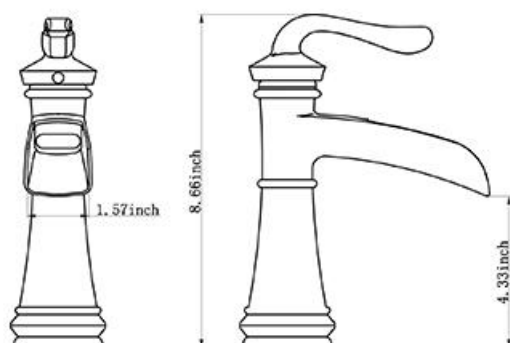
CRITICAL DIMENSIONS
